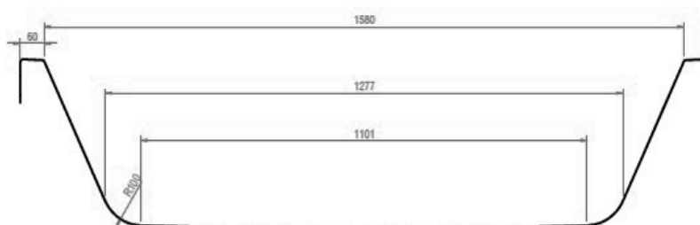
SECTION B-B
