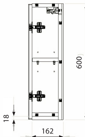
End View
