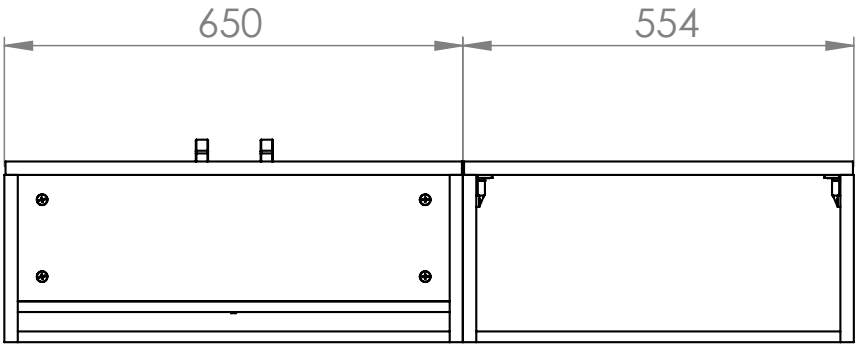
BOTTOM VIEW
