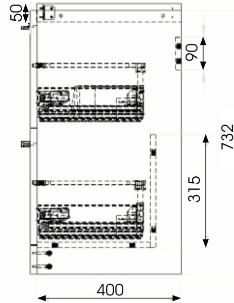
End View
