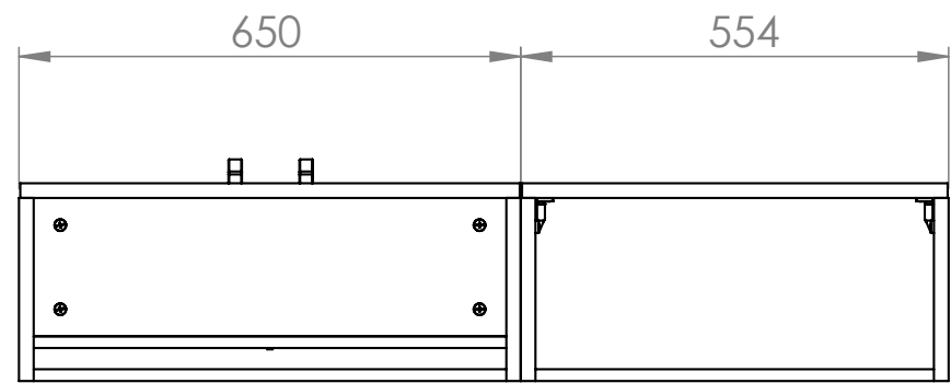
BOTTOM VIEW
