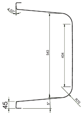
SECTION C-C
